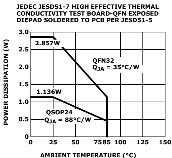
FIGURE 18. PACKAGE POWER DISSIPATION vs AMBIENT TEMPERATURE
