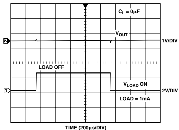
TPC 18. ADR381 Load Transient Response with C_L = 0\mu F
