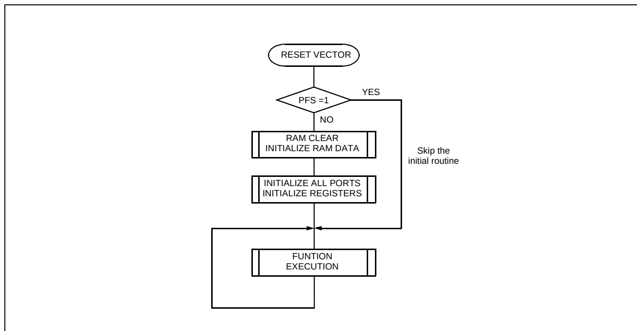
Figure 22-2 Example S/W of RESET by Power fail
