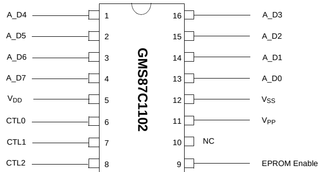
Figure 23-2 Pin Assignment
