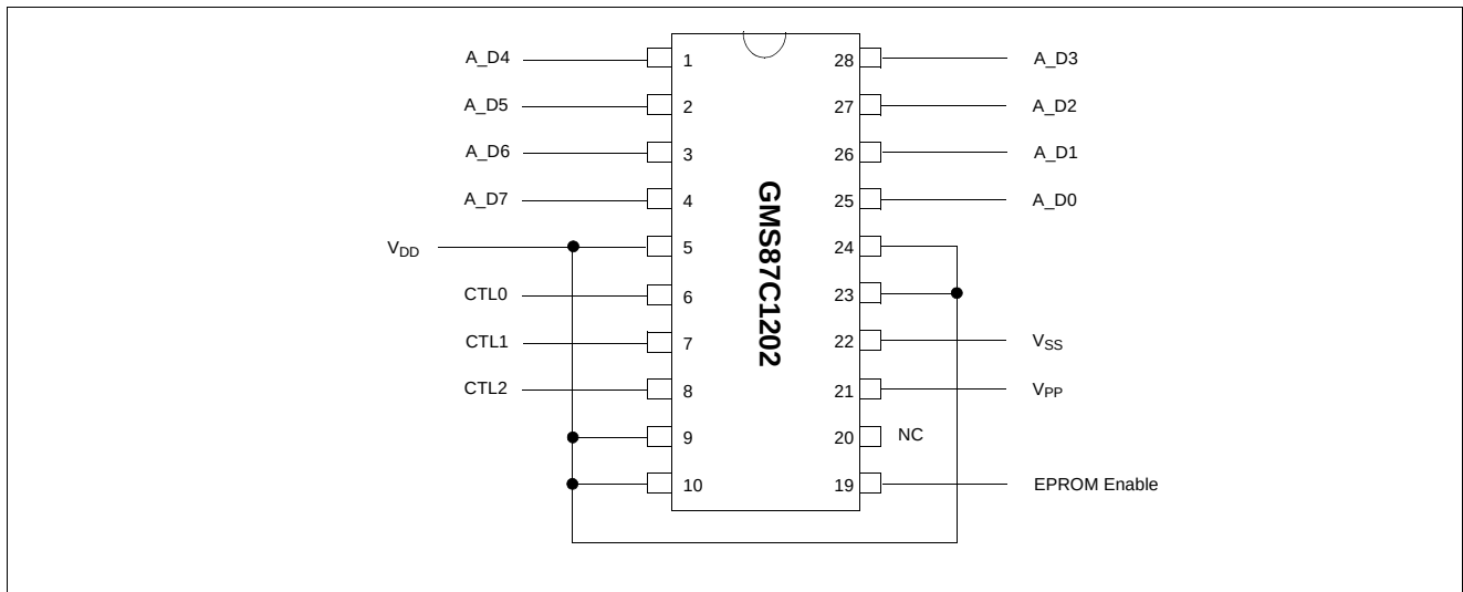
Figure 23-3 Pin Assignment
