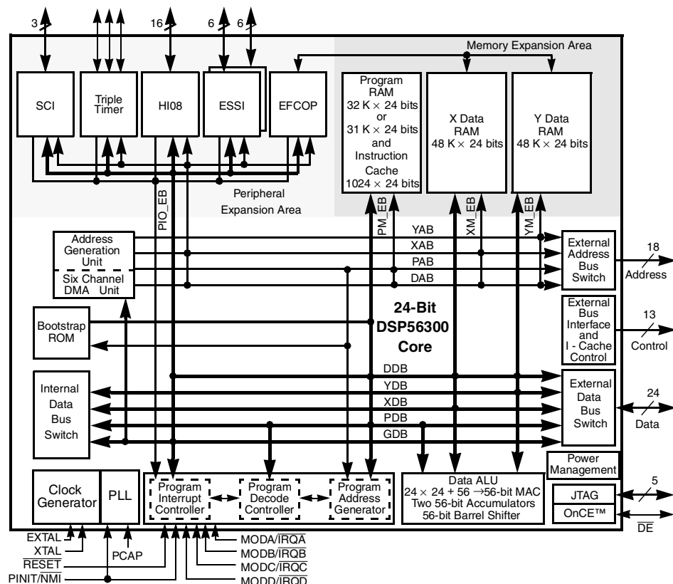
Figure 1. DSP56311 Block Diagram
