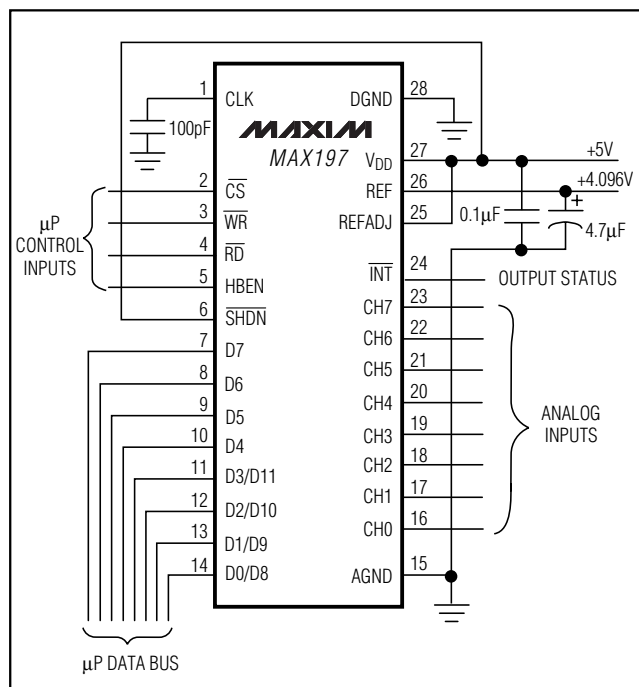
Figure 3. Operational Diagram
