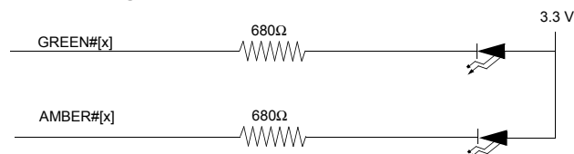
Figure 4. USB Downstream Port Connection
