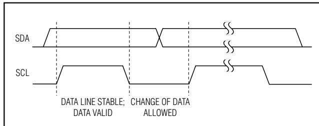
Figure 3. Bit Transfer
