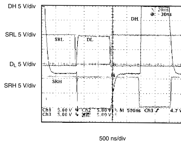
Figure 12. Drive Waveforms
