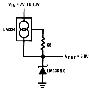
Figure 23. Wide Input Range Reference
