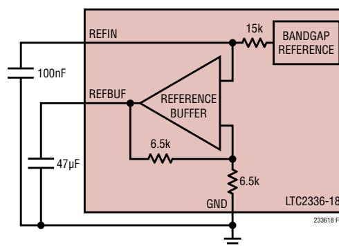
Figure 7a. LTC2336-18 Internal Reference Circuit
