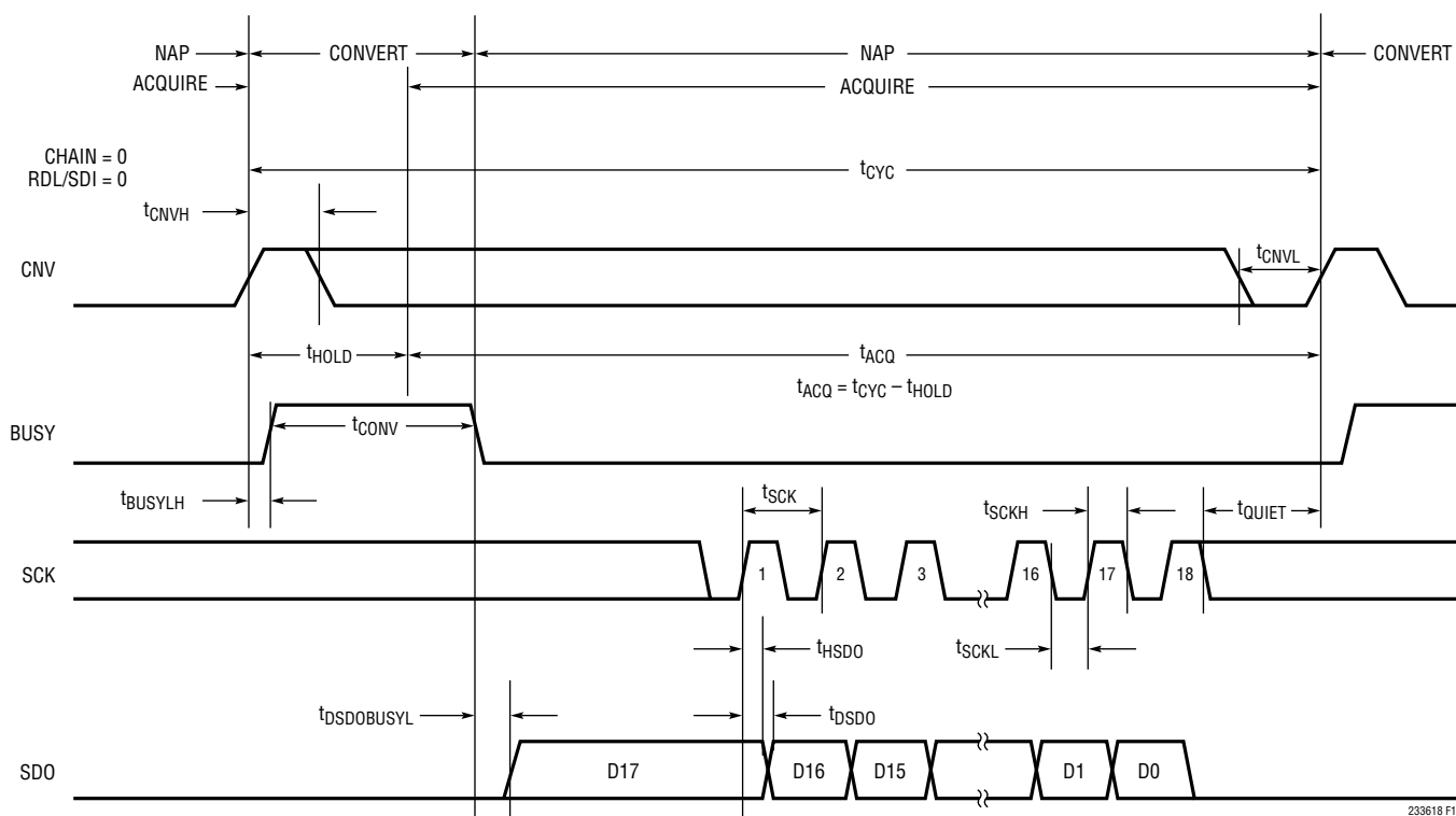
Figure 12. Using a Single LTC2336-18 in Normal Mode
