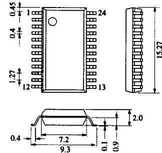
24-Lead PANAFLAT Plastic Package (SO-24D)
