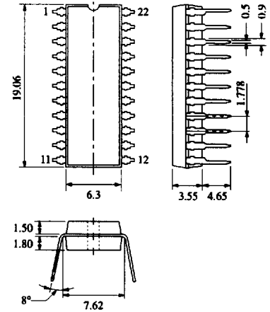
22-Lead Shrink DIP Plastic Package (22-SDIP)
