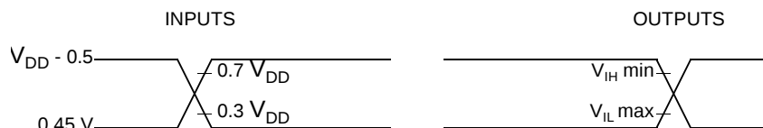
Figure 6-24. AC Testing Input/Output Waveforms
