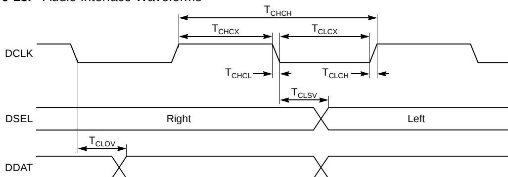
Figure 6-18. Audio Interface Waveforms
