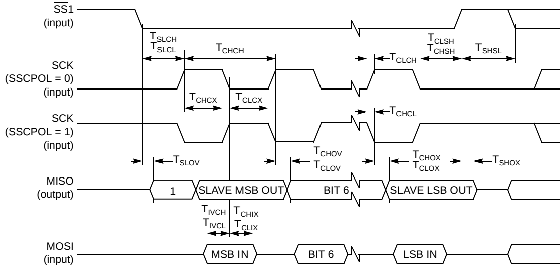
Figure 6-14. SPI Master Waveforms (SSCPHA = 0)
