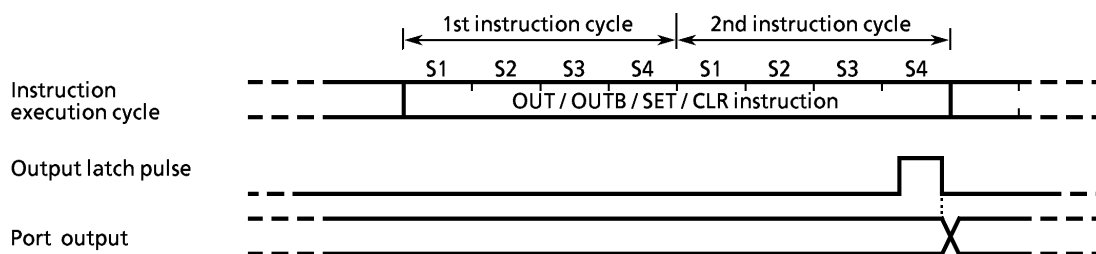
Figure 3-2. Output Timing
