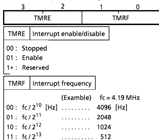
Figure 3-9. Interval Timer Interrupt Command Register
