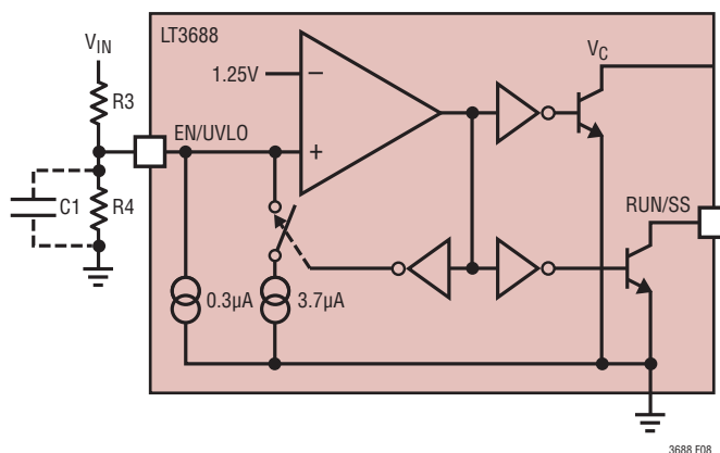
Figure 8. Undervoltage Lockout
