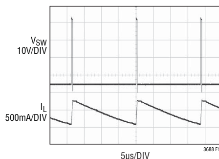
Figure 12. The LT3688 Reduces Its Frequency to Below 70kHz to Protect Against Shorted Output with 36V Input
