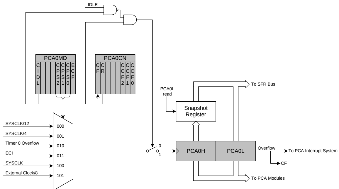
Figure 34.2. PCA Counter/Timer Block Diagram
