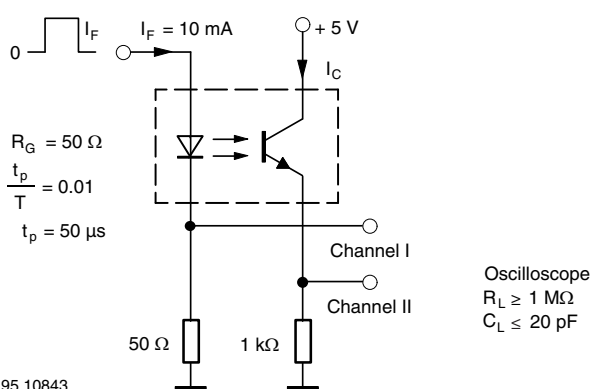
Fig. 3 - Test Circuit, Saturated Operation
