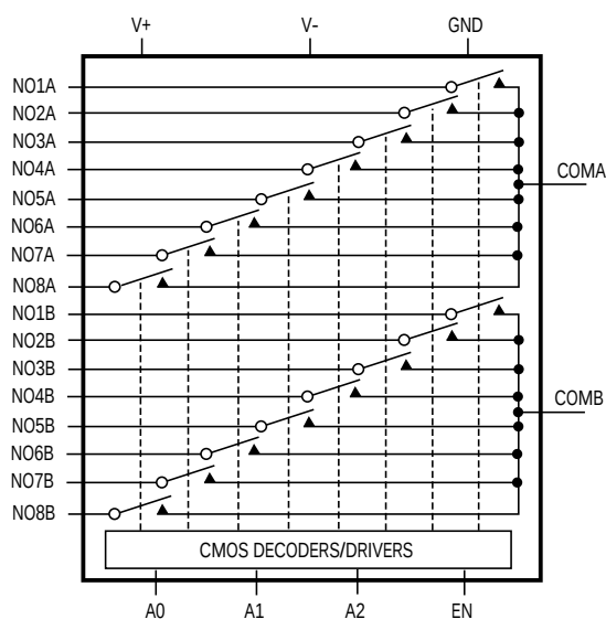
MAX337 8-CHANNEL DIFFERENTIAL MULTIPLEXER
