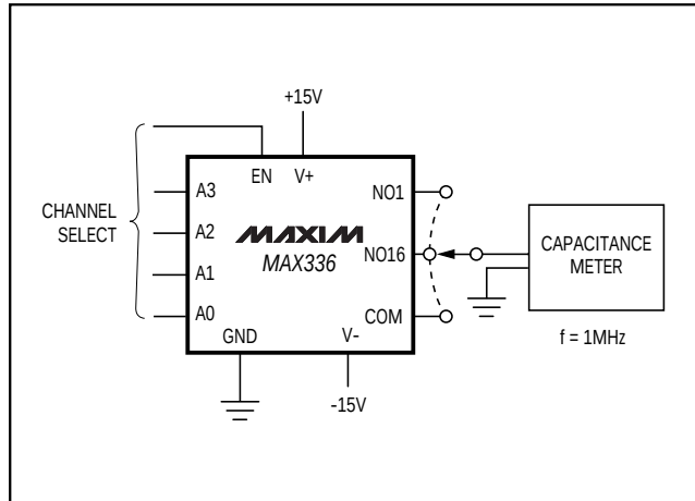
Figure 8. NO/COM Capacitance
