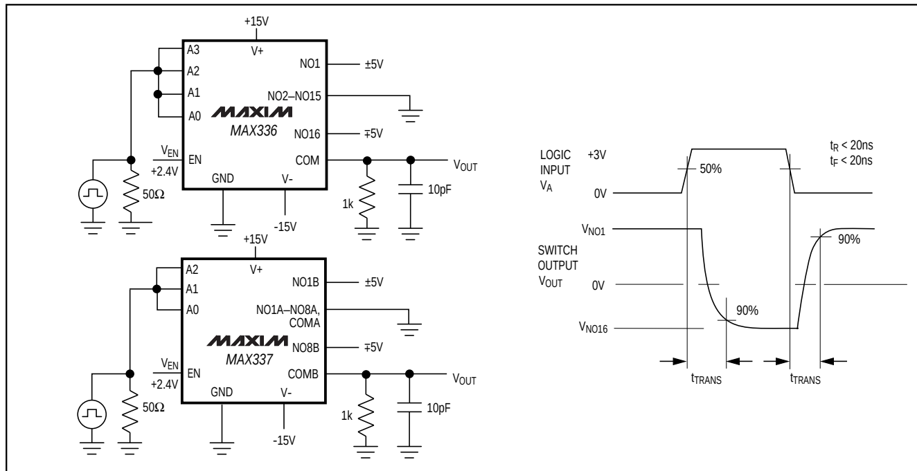
Figure 2. Transition Time
