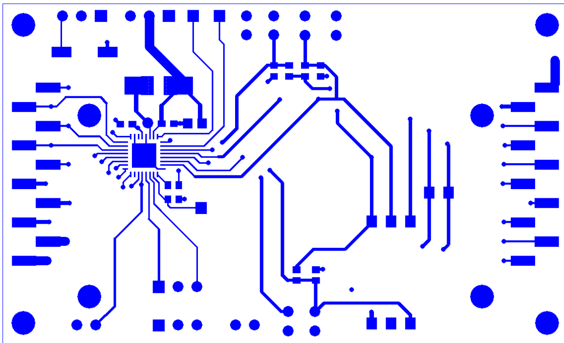
Figure 7: 73S8009C Demo Board: Top Signal Layer
