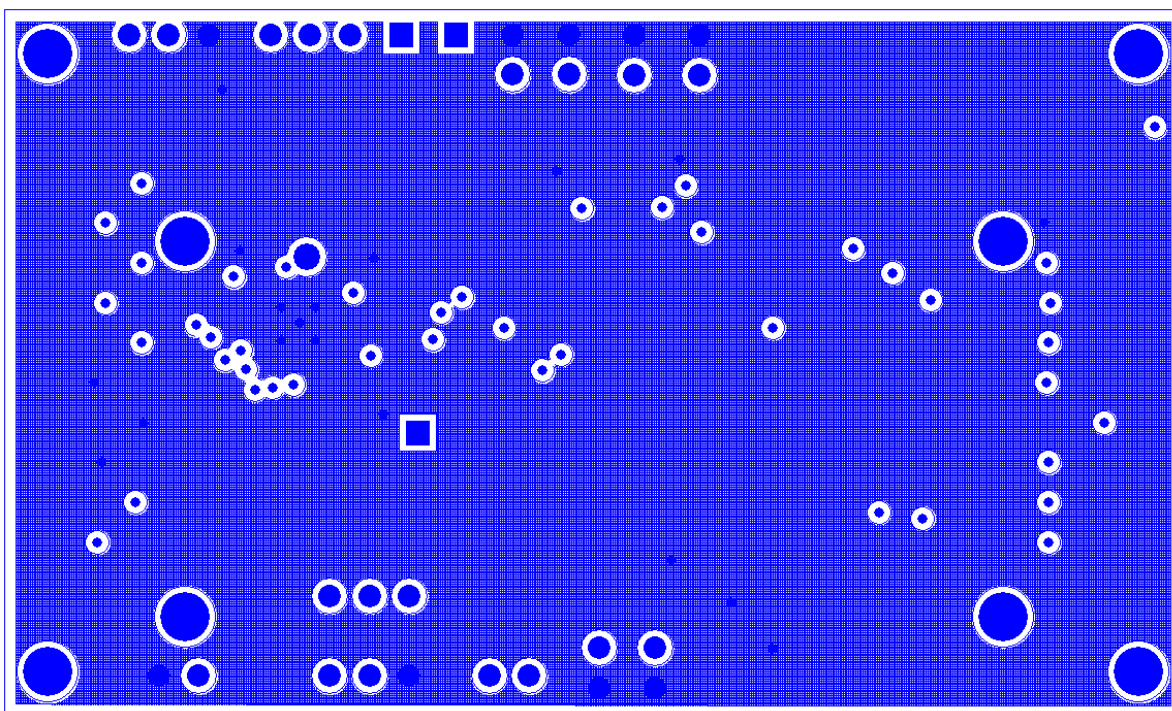
Figure 8: 73S8009C Demo Board: Middle Layer 1, Ground Plane
