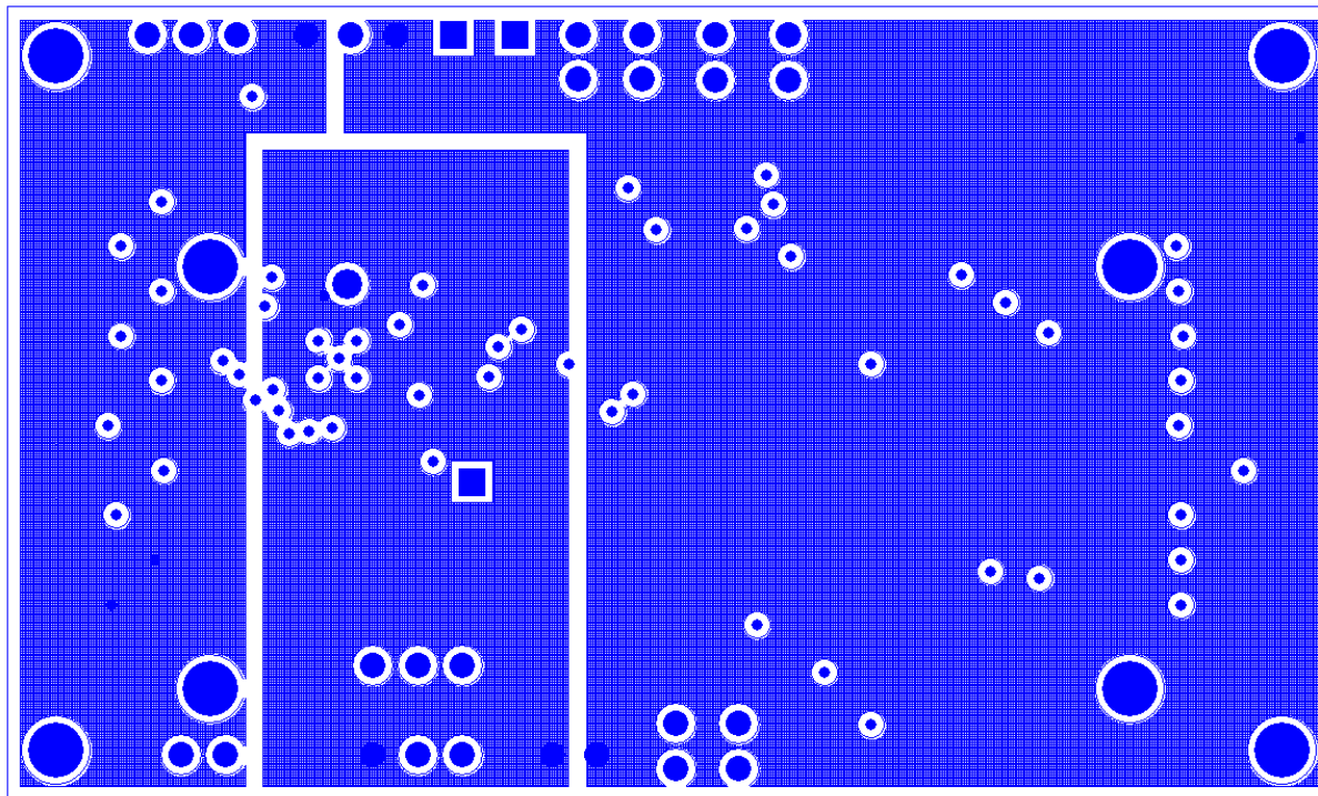
Figure 9: 73S8009C Demo Board: Middle Layer 2, Supply Plane
