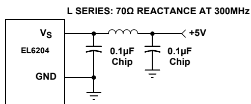
FIGURE 22. RECOMMENDED SUPPLY BYPASSING
