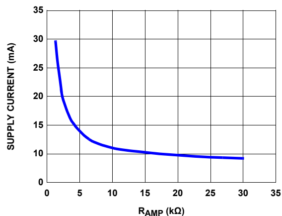
FIGURE 10. SUPPLY CURRENT vs R_{AMP}
