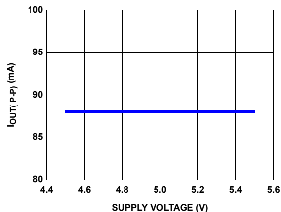
FIGURE 12. PEAK-TO-PEAK OUTPUT CURRENT vs SUPPLY VOLTAGE
