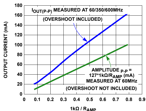
FIGURE 8. OUTPUT CURRENT vs 1/R_{AMP}
