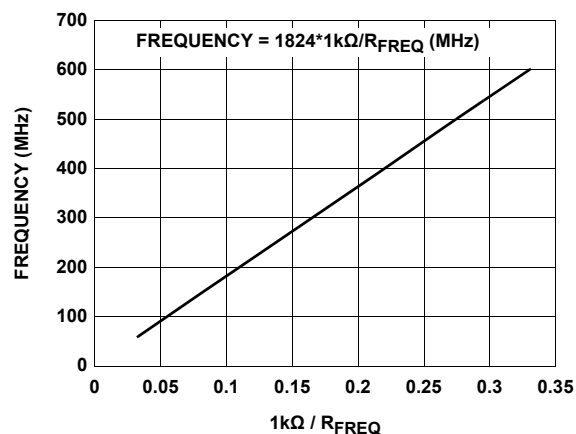
FIGURE 6. FREQUENCY vs 1/R_{FREQ}
