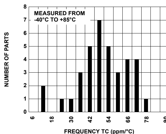
FIGURE 4. FREQUENCY DRIFT WITH TEMPERATURE
