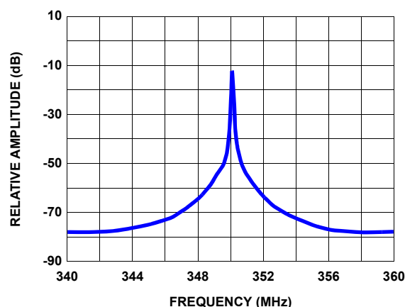
FIGURE 20. OUTPUT SPECTRUM-WIDEBAND
