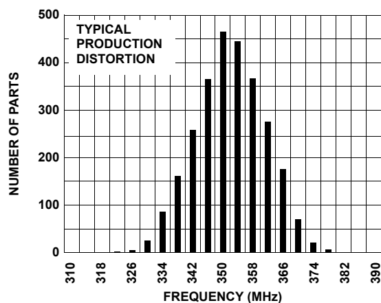
FIGURE 3. FREQUENCY DISTRIBUTION
