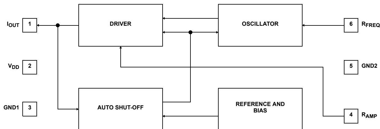
FIGURE 1. BLOCK DIAGRAM
