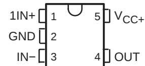
LMV321 . . . DBV PACKAGE (TOP VIEW)
