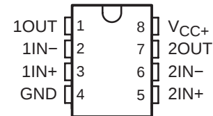
LMV358 . . . D OR PW PACKAGE (TOP VIEW)
