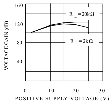
Figure 16. Voltage gain
