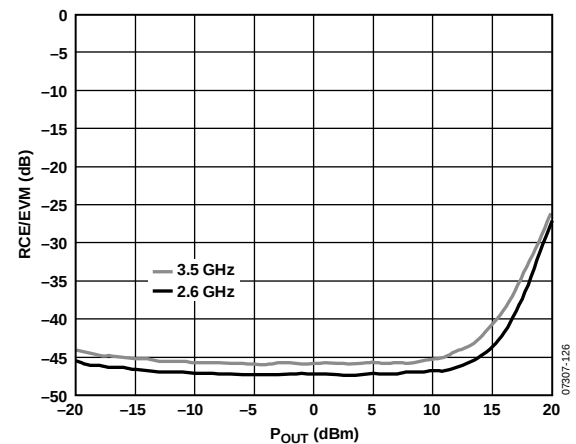
Figure 34. RCE/EVM vs. P_{\text{OUT}} , WiMAX 64 QAM, 10 MHz Bandwidth, Single Carrier
