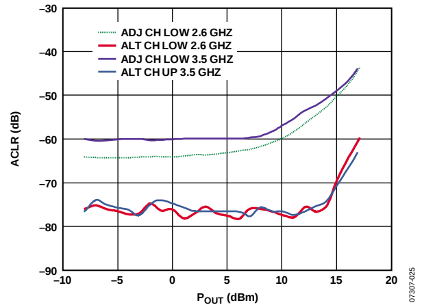
Figure 33. ACLR vs. P_{\text{OUT}} , WiMAX 64 QAM, 10 MHz Bandwidth, Single Carrier
