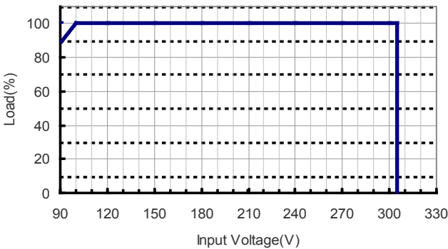
Derating Curve
