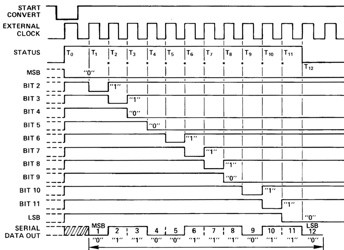
Figure 3. Timing Diagram
