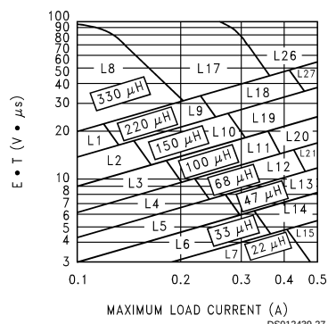
FIGURE 7. LM2594/LM2594HV-ADJ
