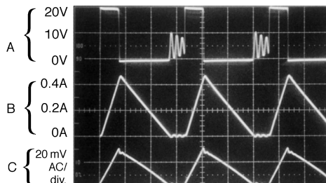
A: Output Pin Voltage, 10V/div. B: Inductor Current 0.2A/div. C: Output Ripple Voltage, 20 mV/div.
