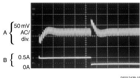
A: Output Voltage, 50 mV/div. (AC) B: 200 mA to 500 mA Load Pulse
