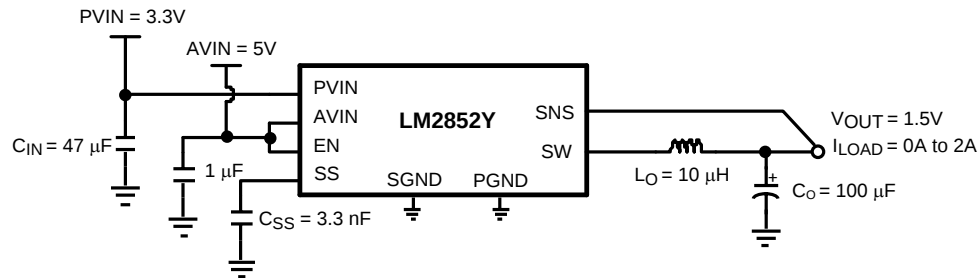
Figure 12. Split-Rail Operation
