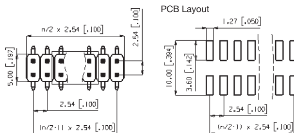
PCB Layout
