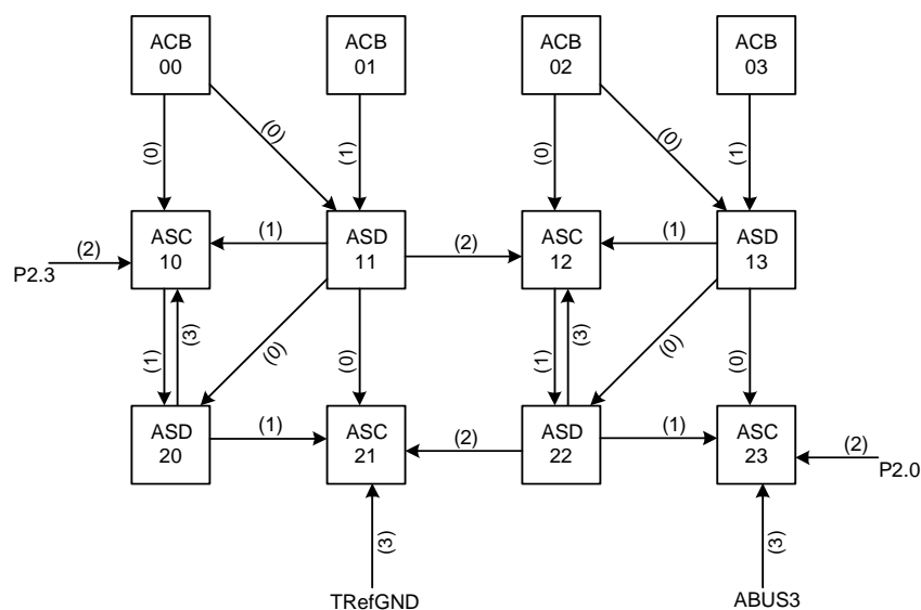
Figure 19-6. BMuxSC/SD Connections
