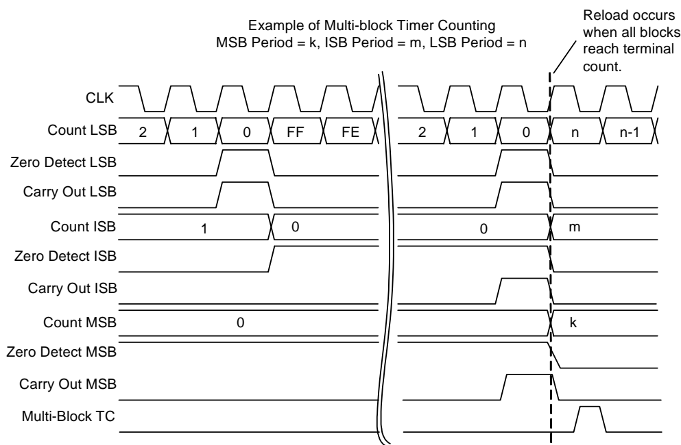
Figure 17-6. Multi-Block Timing
