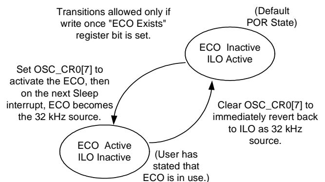
Figure 10-1. State Transition Between ECO and ILO Operation
