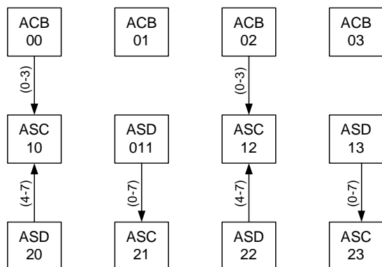
Figure 19-5. CMux Connections
