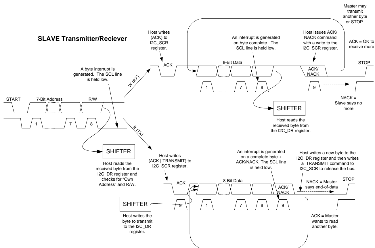
Figure 27-2. Slave Operation
