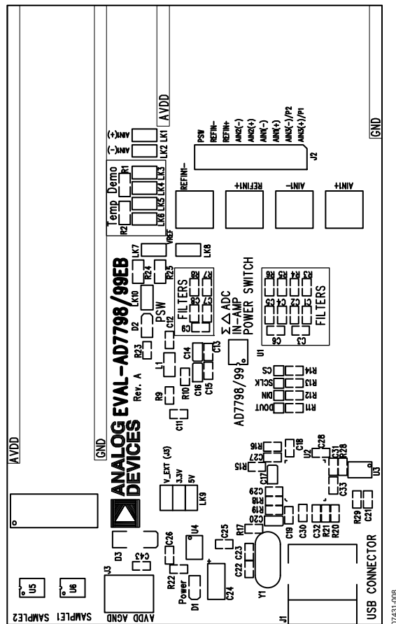
Figure 8. AD7799 Evaluation Board—Component Layout Diagram
