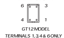
TERMINAL NOS. FOR REFERENCE ONLY
