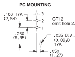
PC MOUNTING
