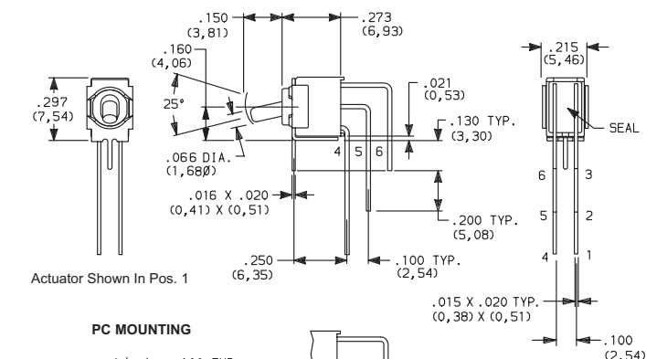
PART NUMBER SWITCH FUNCTION POS.1 POS. 2 POS. 3 GT 21MAVBE GT 23MAVBE ON ON NONE OFF ON ON Conn. Terms. 2-3 5-6 OPEN 2-1, 5-4 Schematic DPDT GT 22MAVBE OFF NONE ON Conn. Terms. OPEN N/A 3-1, 6-4 Schematic DPST
