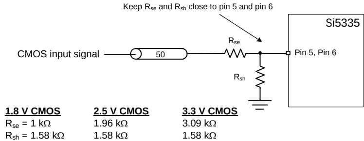
Figure 13. P5, P6 Control Pin Termination
