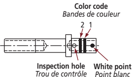
Female Contact / Contact femelle
