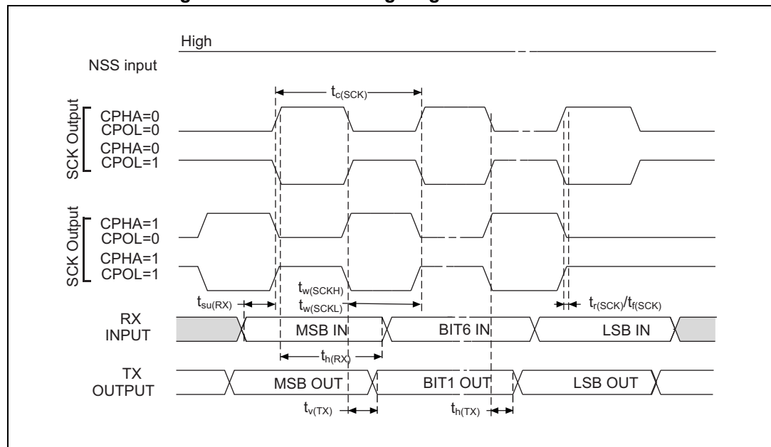
Figure 100. USART timing diagram in Master mode
