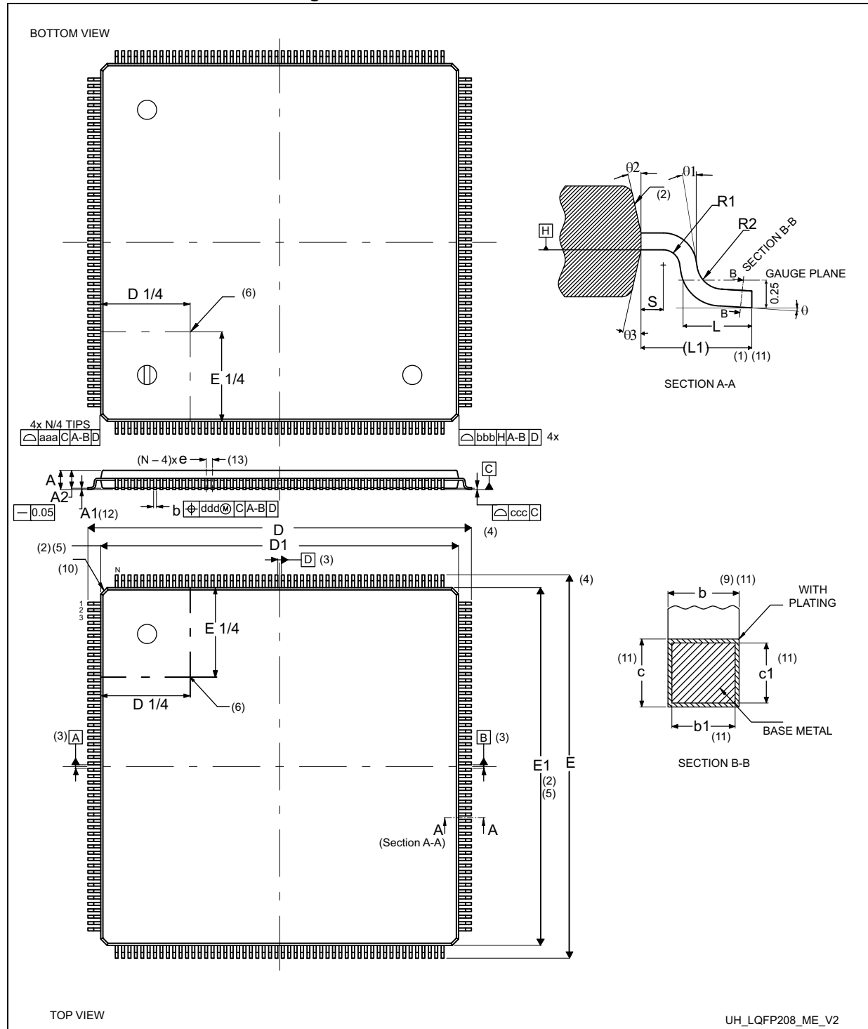
Figure 129. LQFP208 - Outline (15)
