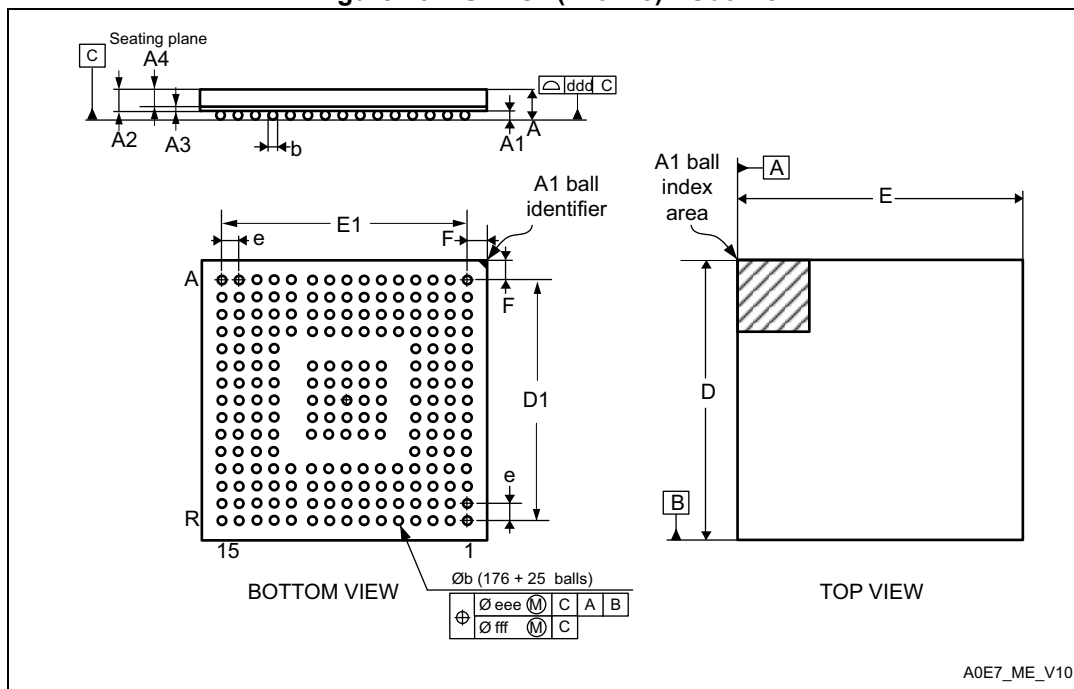
Figure 131. UFBGA(176+25) - Outline
