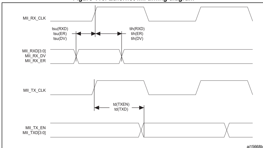
Figure 116. Ethernet MII timing diagram
