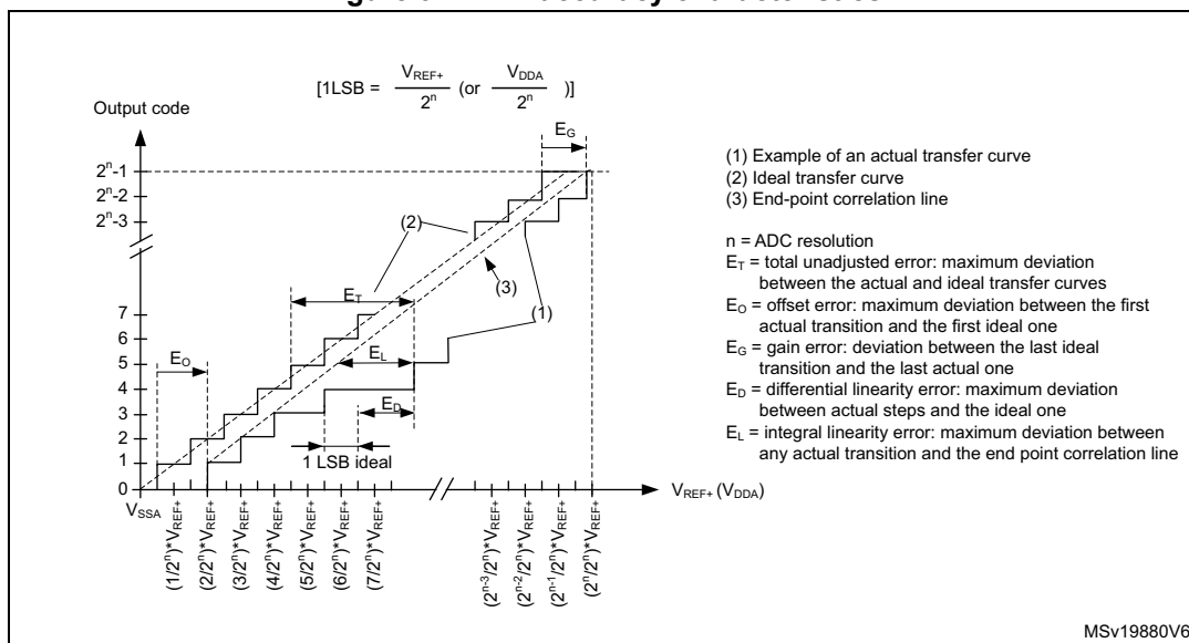
Figure 91. ADC accuracy characteristics
