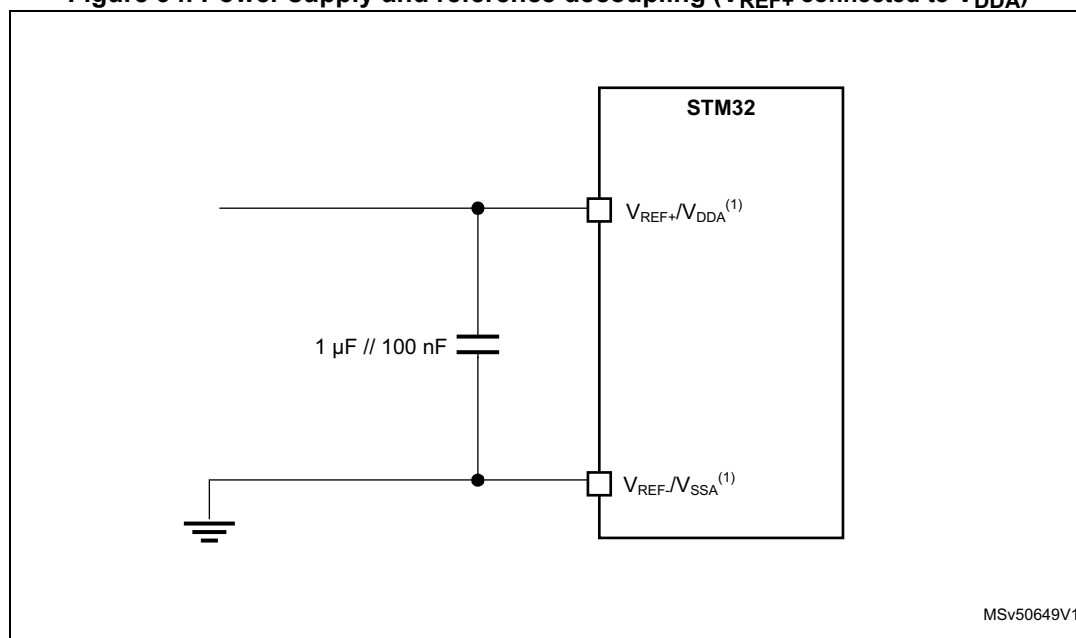
Figure 94. Power supply and reference decoupling ( V_{REF+} connected to V_{DDA} )
