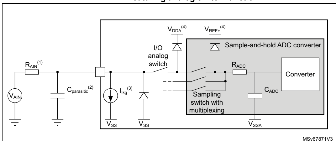
Figure 92. Typical connection diagram when using the ADC with FT/TT pins featuring analog switch function
