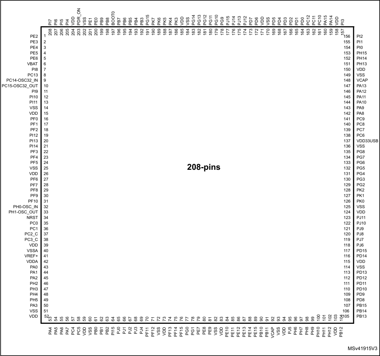
Figure 10. LQFP208 pinout
