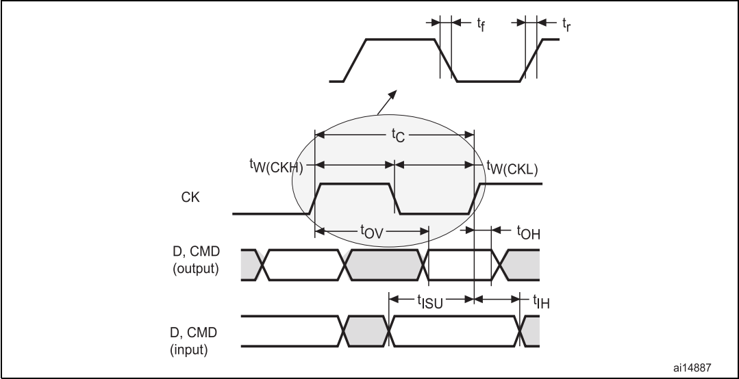
Figure 110. SDIO high-speed mode
