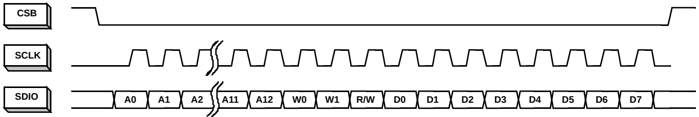
FIGURE 36. LSB-FIRST ADDRESSING
