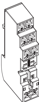
Standard model
