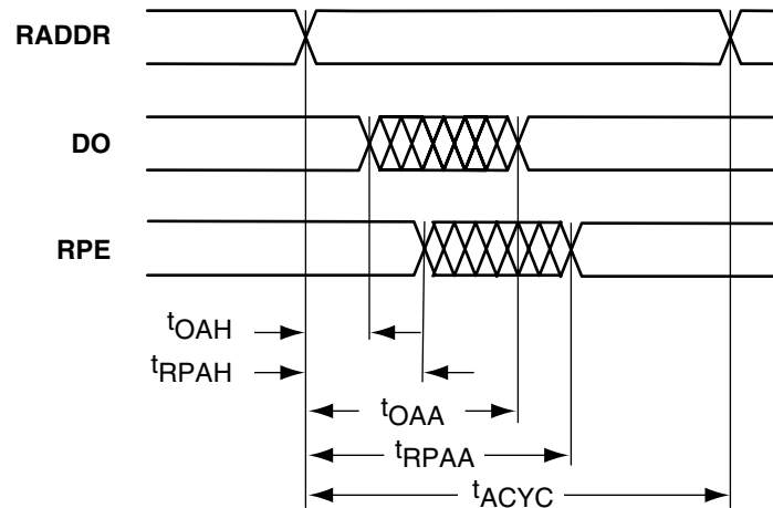
Figure 2-31 • Asynchronous SRAM Read, Address Controlled, RDB = 0
