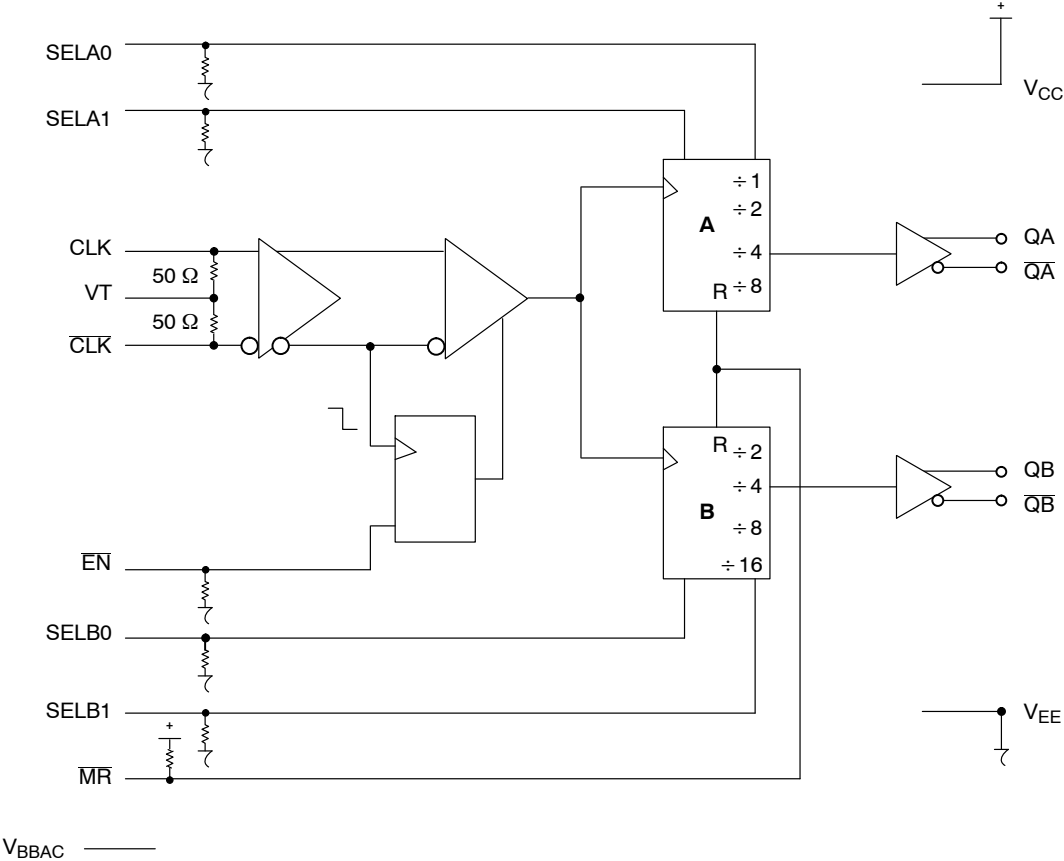
Figure 3. Logic Diagram
