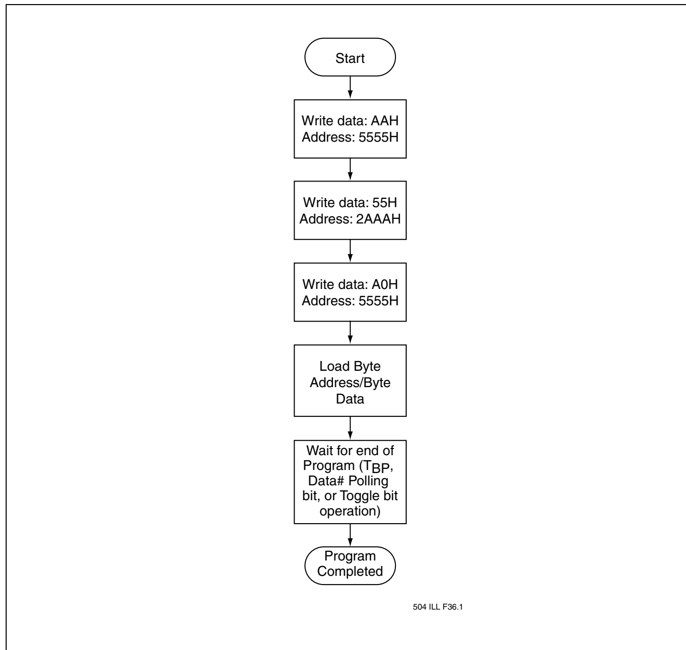
FIGURE 26: BYTE-PROGRAM ALGORITHM
