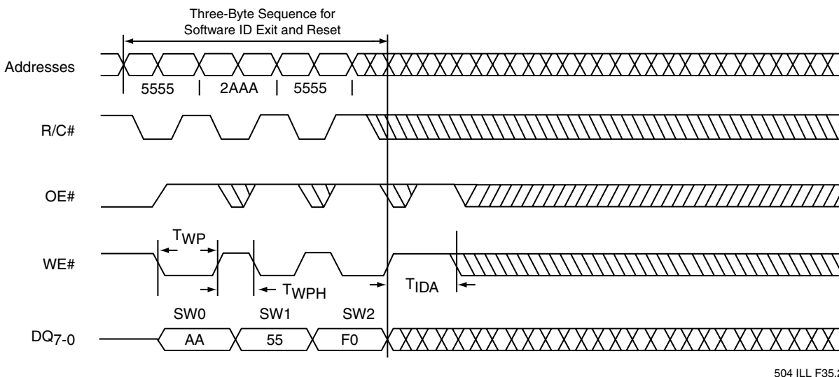
FIGURE 23: SOFTWARE ID EXIT AND RESET (PP MODE)
