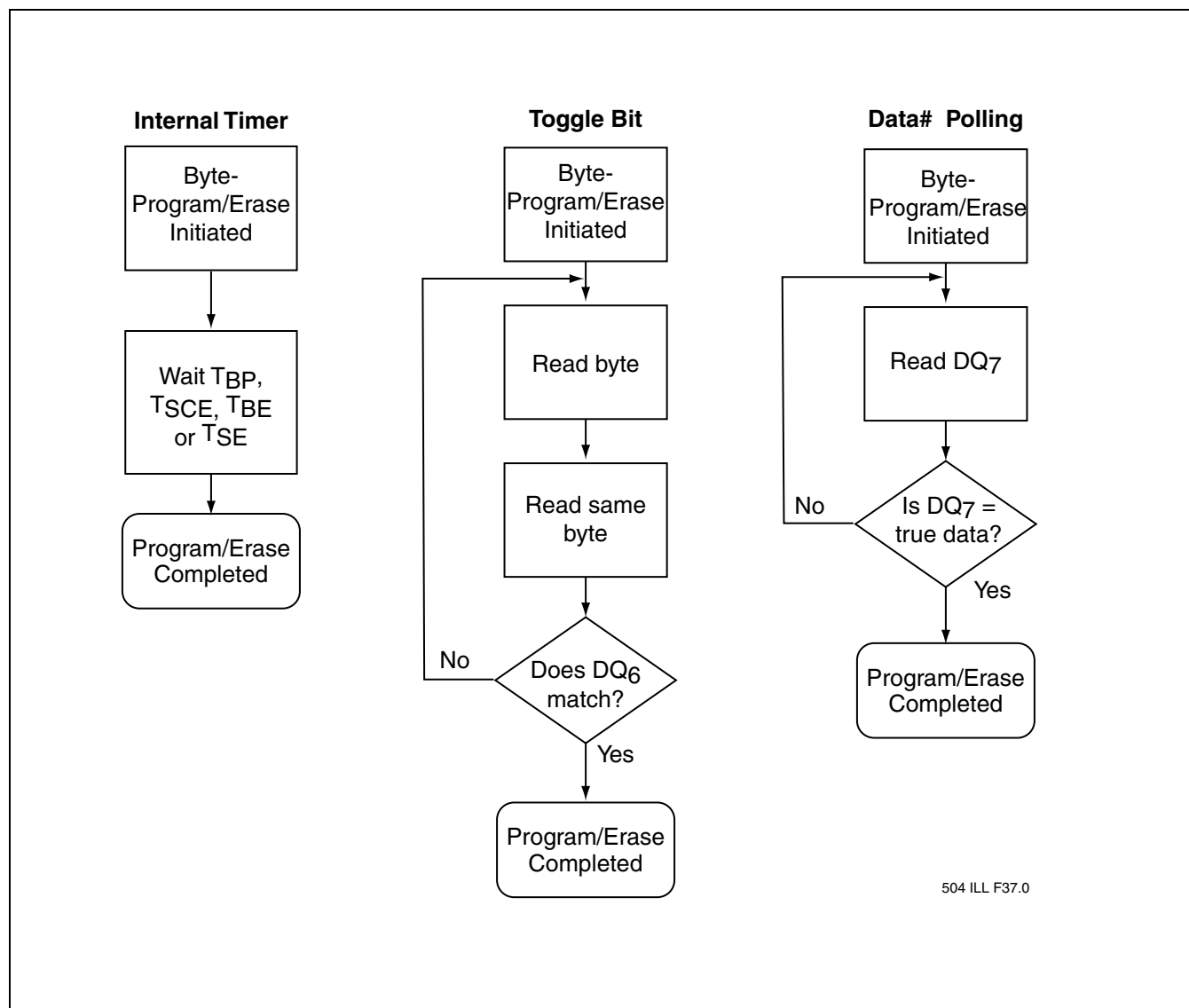
FIGURE 27: WAIT OPTIONS
