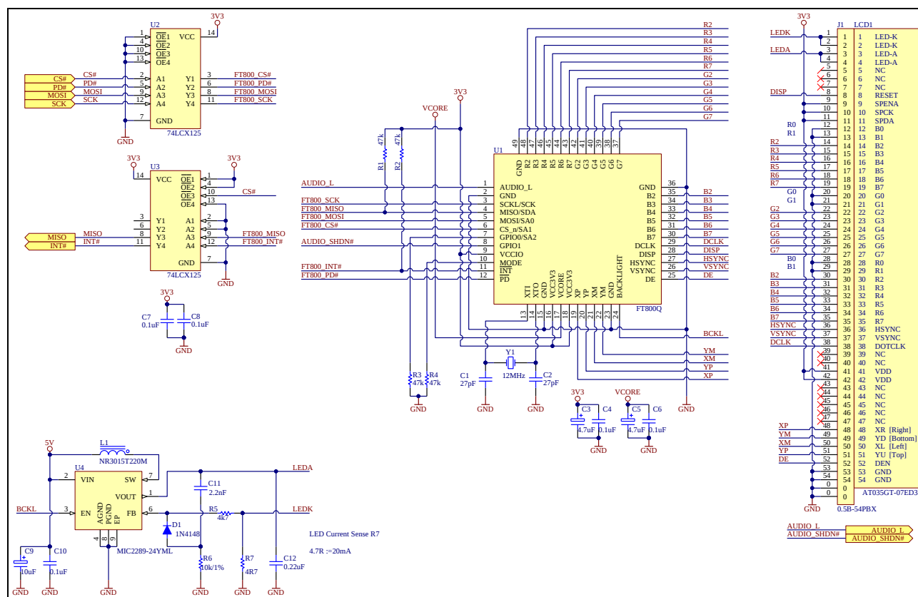
Figure 4-1 - VM800B35A (3.5" Version)
