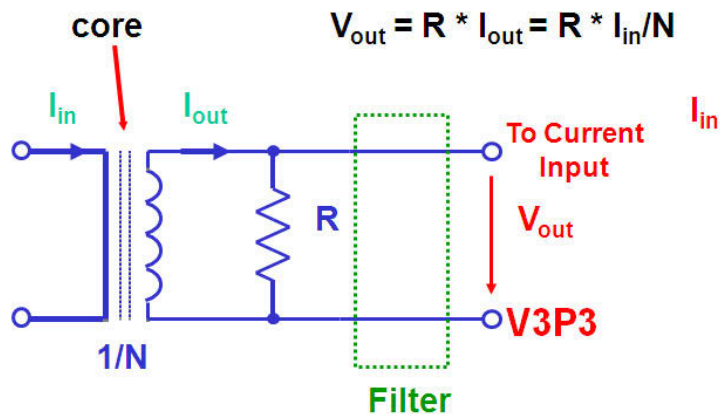
Figure 9: Current Transformer
