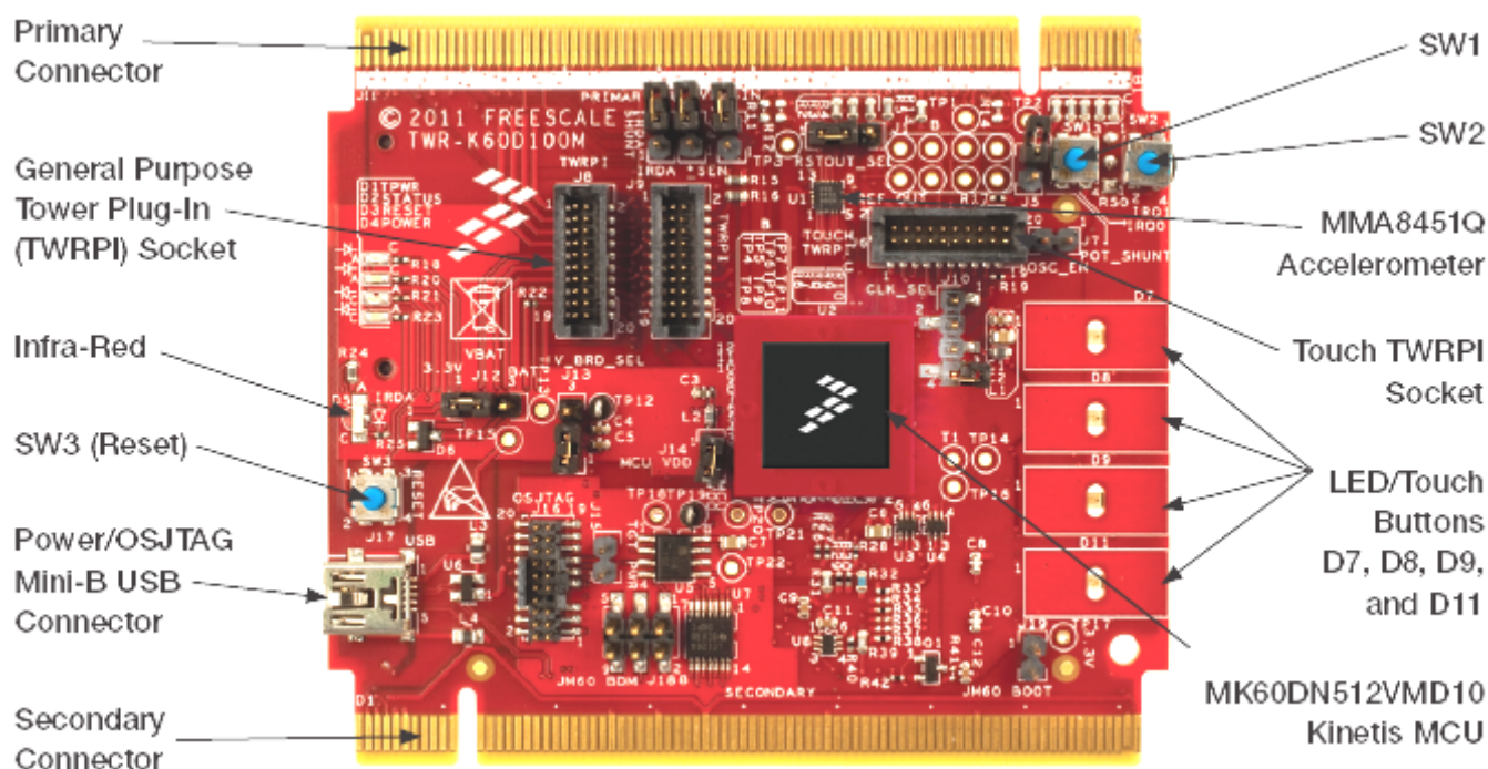
Figure 2. Callouts on front side of the TWR-K60D100M
