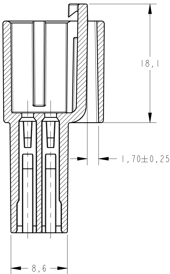
SECTION B-B
