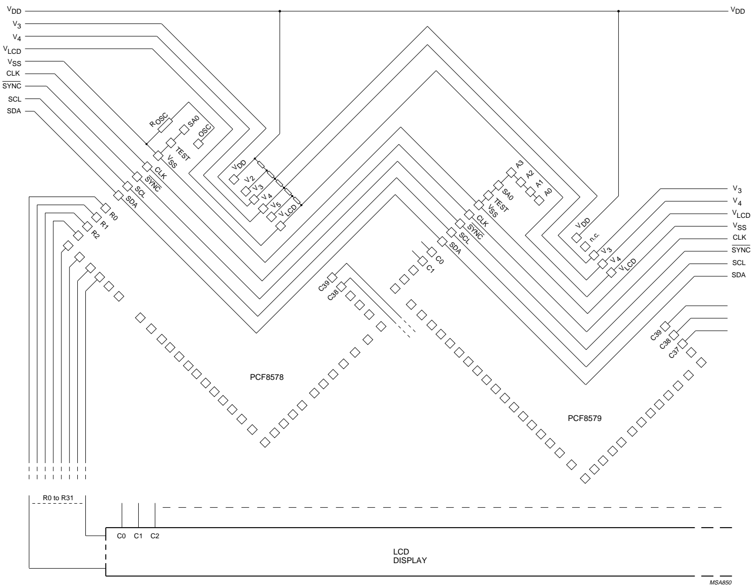
Fig.29 Typical chip-on glass application (viewed from the underside of the chip).
