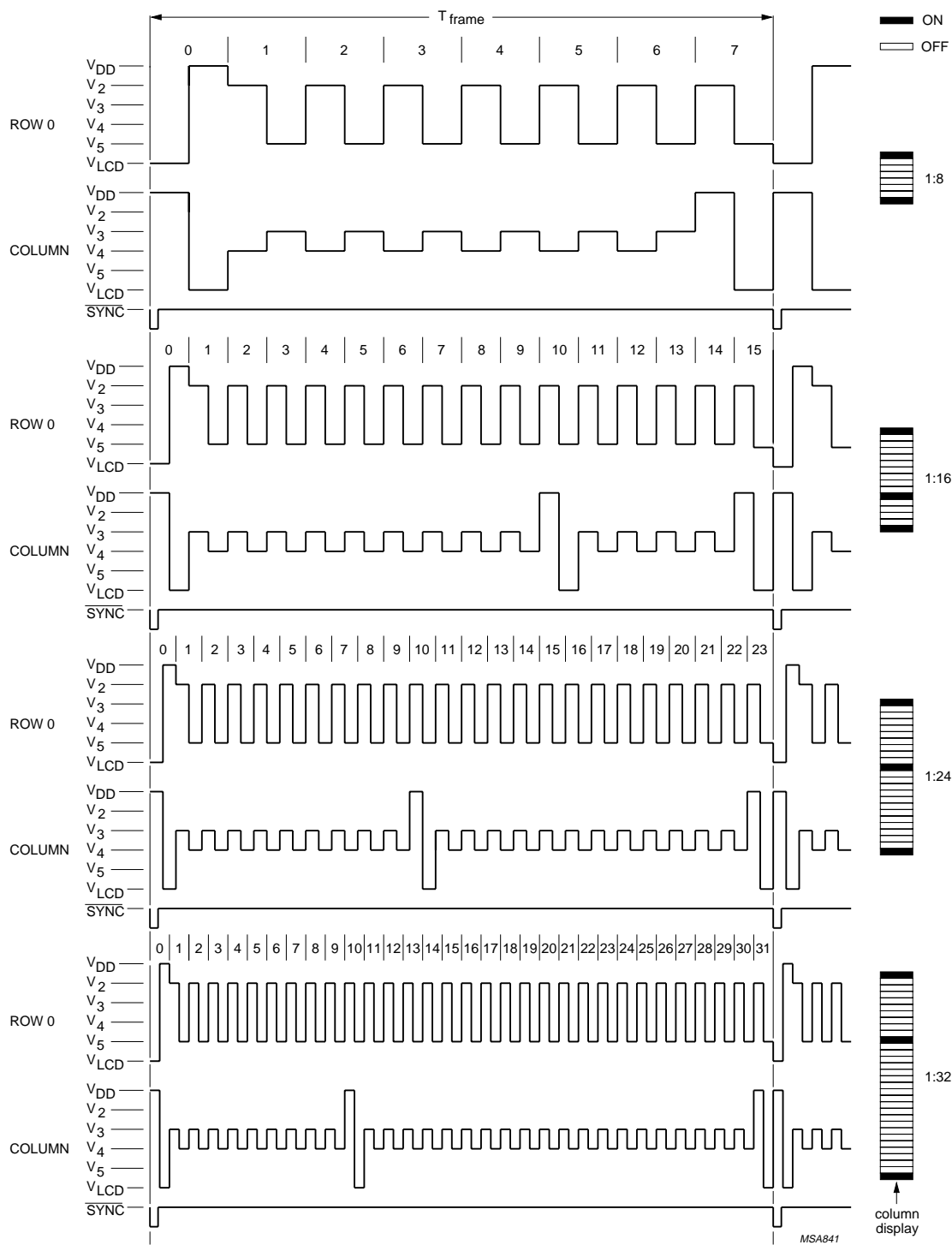
Fig.6 LCD row/column waveforms.
