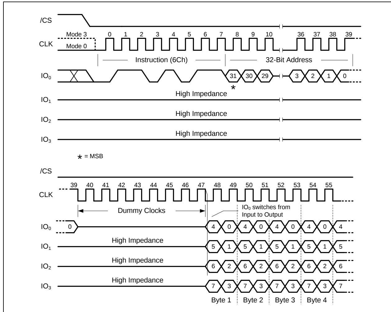
Figure 21. Fast Read Quad Output with 4-Byte Address Instruction (SPI Mode only)
