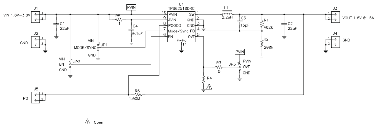
Figure 10. TPS62510EVM-168 Schematic
