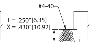
FLUSH MOUNTING WITH THREADED INSERT (T, X)
