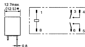
Terminal Arrangement/ Internal Connection (Bottom View)
