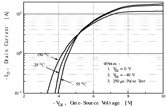
Fig 2. Transfer Characteristics
