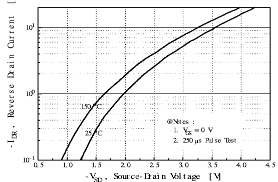
Fig 4. Source-Drain Diode Forward Voltage
