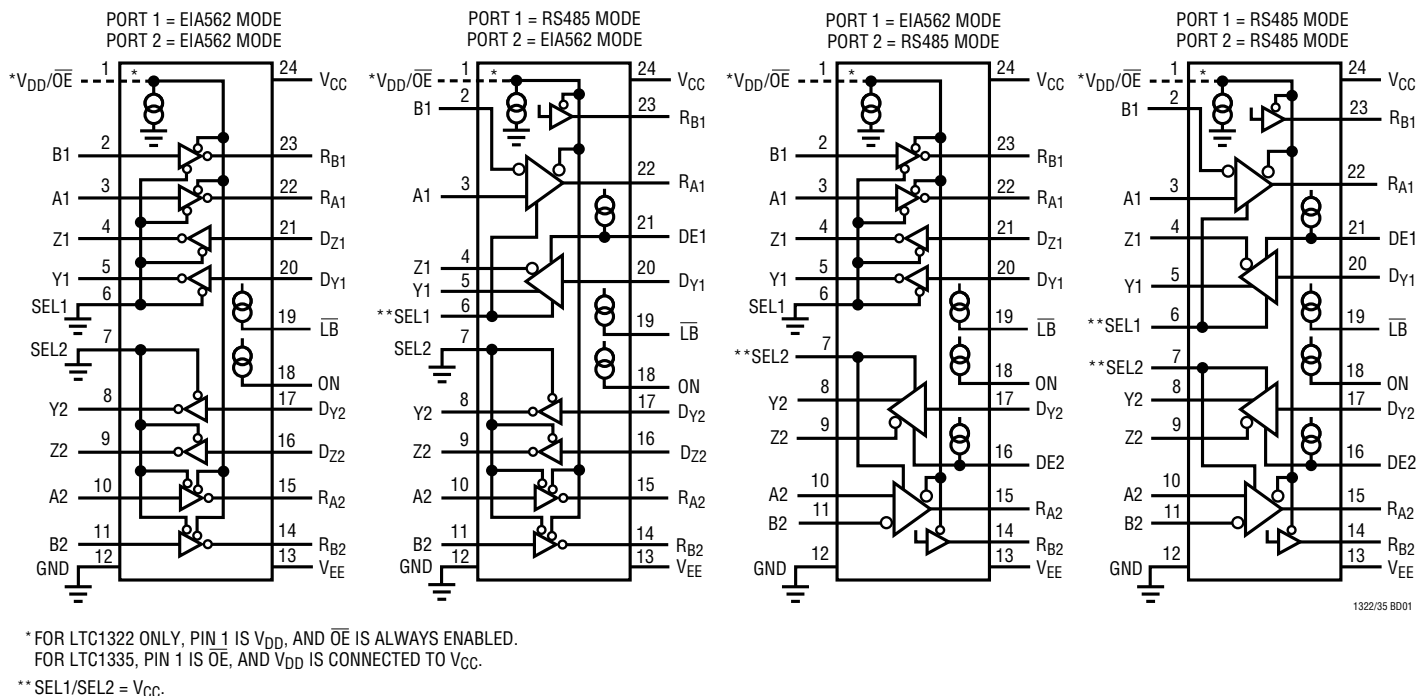
LTC1322/LTC1335 Interface Configuration Without Loopback
