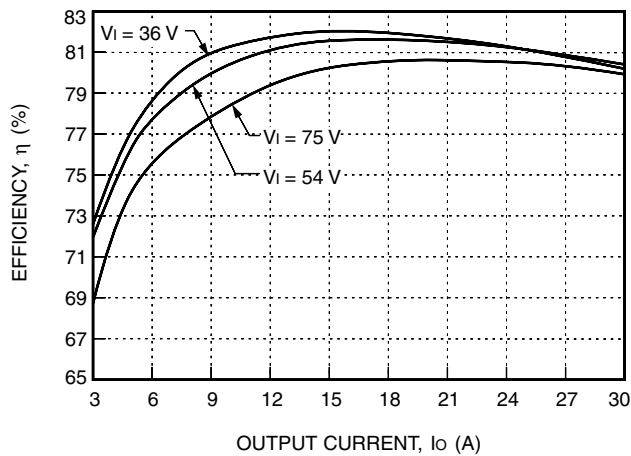
Figure 12. Typical JFW150F Converter Efficiency vs. Output Current at Room Temperature
